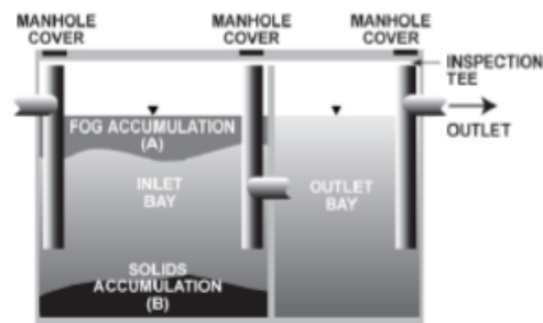
Grease Interceptor (Outside)
