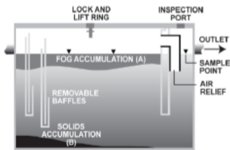
Grease Trap/Hydro-mechanical (inside/outside)
